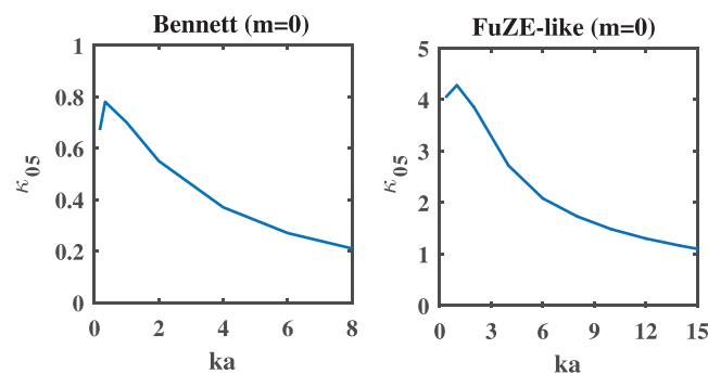
FIG. 7. Dimensionless shear strength \kappa_{05} needed to suppress m=0 growth rate to 0.05/t_a for Bennett (left) and FuZE-like (right) profiles with u_{20}/v_i = \kappa r/a .
