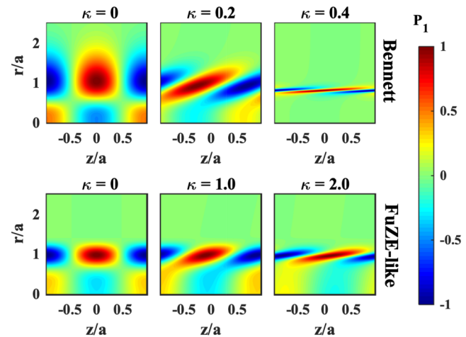
FIG. 6. Effect of non-dimensional shear strength \kappa on pressure perturbation for m=0 sausage modes using Bennett (top) and FuZE-like (bottom) profiles with ka=10/3 and u_{z0}/v_i = \kappa r/a .
